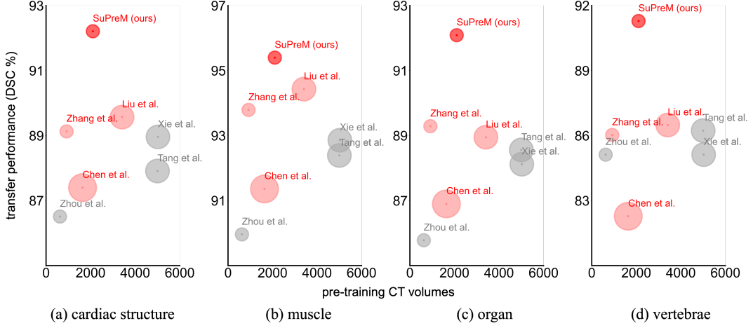
Figure 8: A comprehensive benchmark on supervised and self-supervised models. We present the segmentation performance achieved by fine-tuning models using the entire TotalSegmentator training set ( N = 1081 annotated CT volumes) as target tasks. A larger circle size denotes a greater number of model parameters. Overall, for target tasks, supervised models (in red) transfer better for pre-training in comparison with self-supervised models (in gray). Detailed per-class performance can be found in Appendix Table 9.
